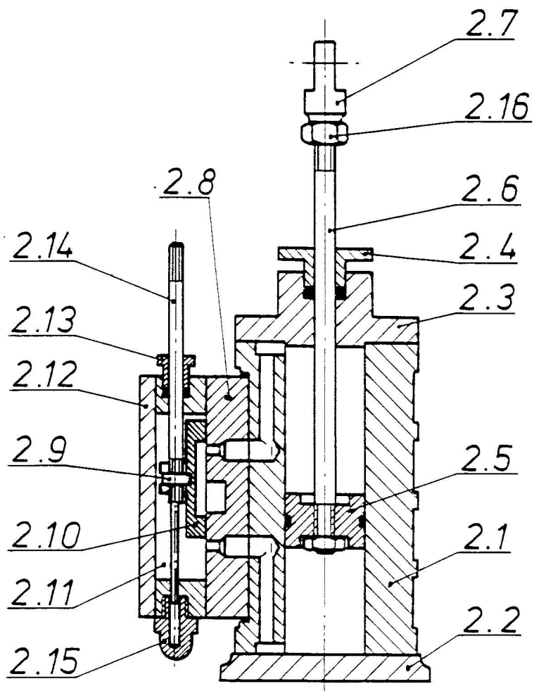
Cylinder and Steam Chest
