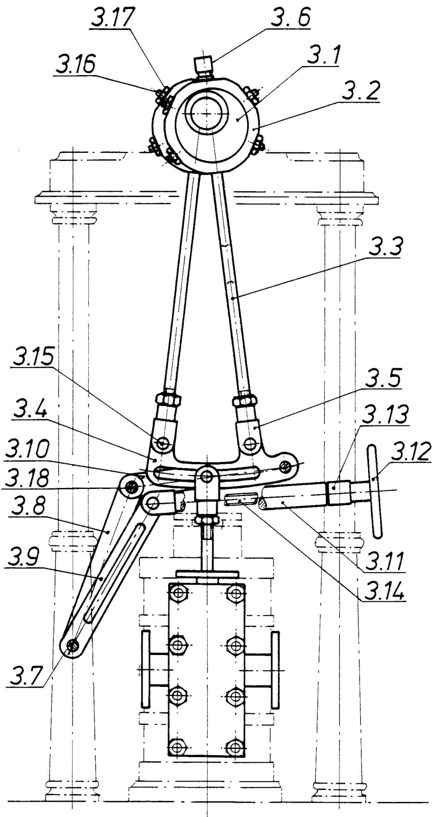
Valve Gear
