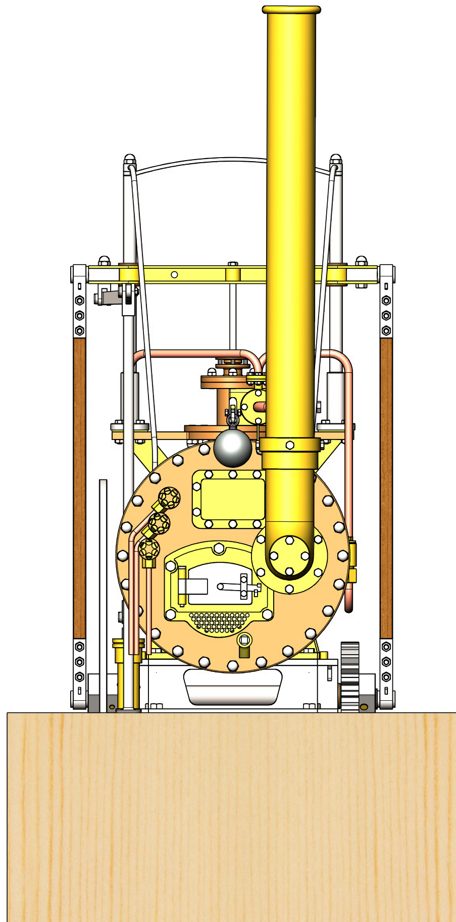
FRONT VIEW
