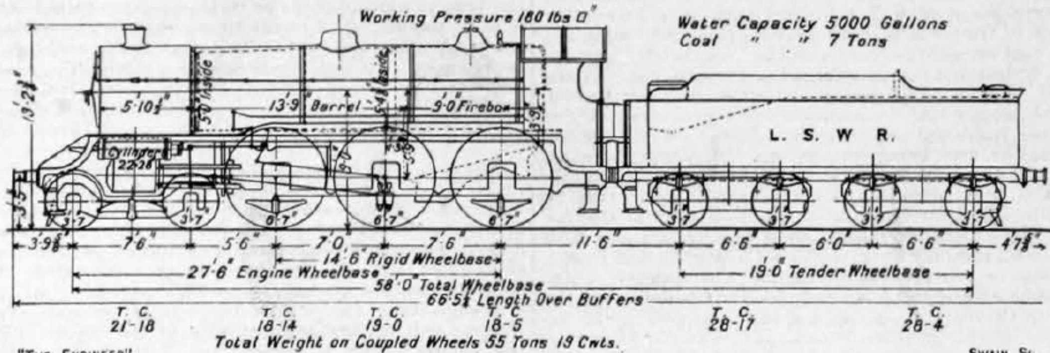
WEIGHT DIAGRAM OF SIX-COUPLED PASSENGER ENGINE
