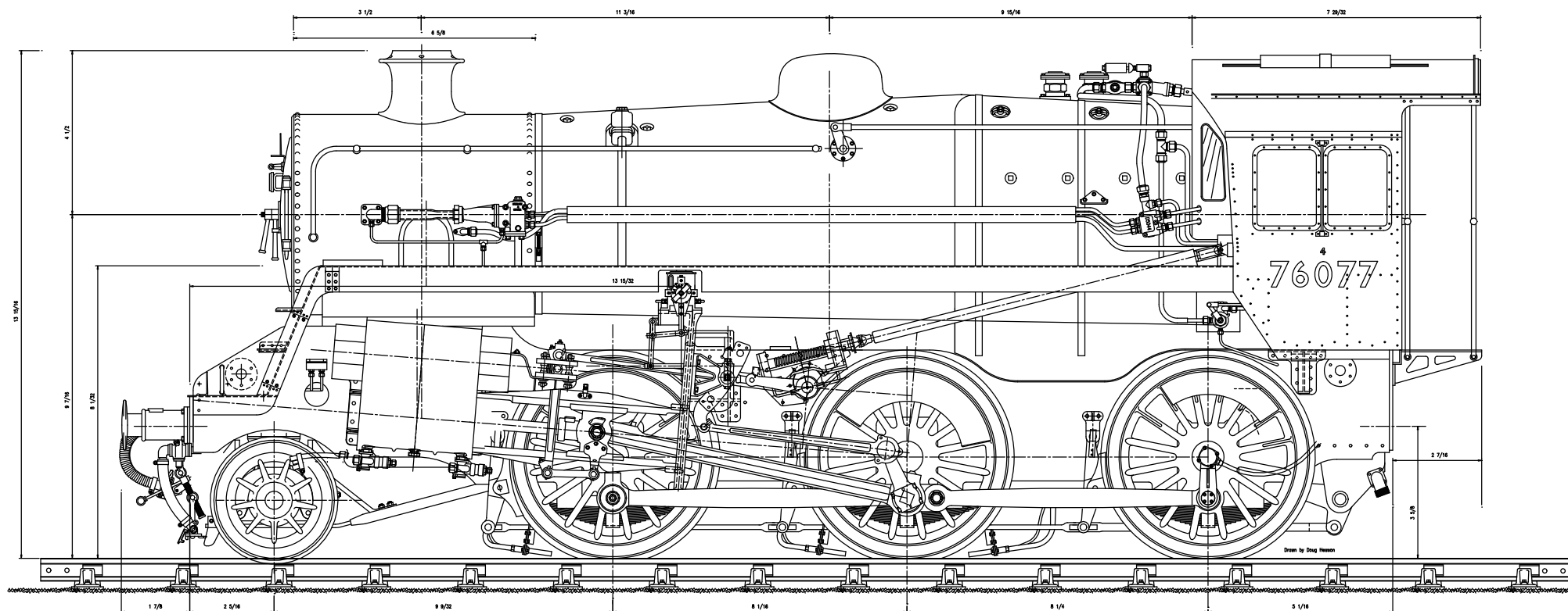
GENERAL ARRANGEMENT DRAWING L.H. SIDE
