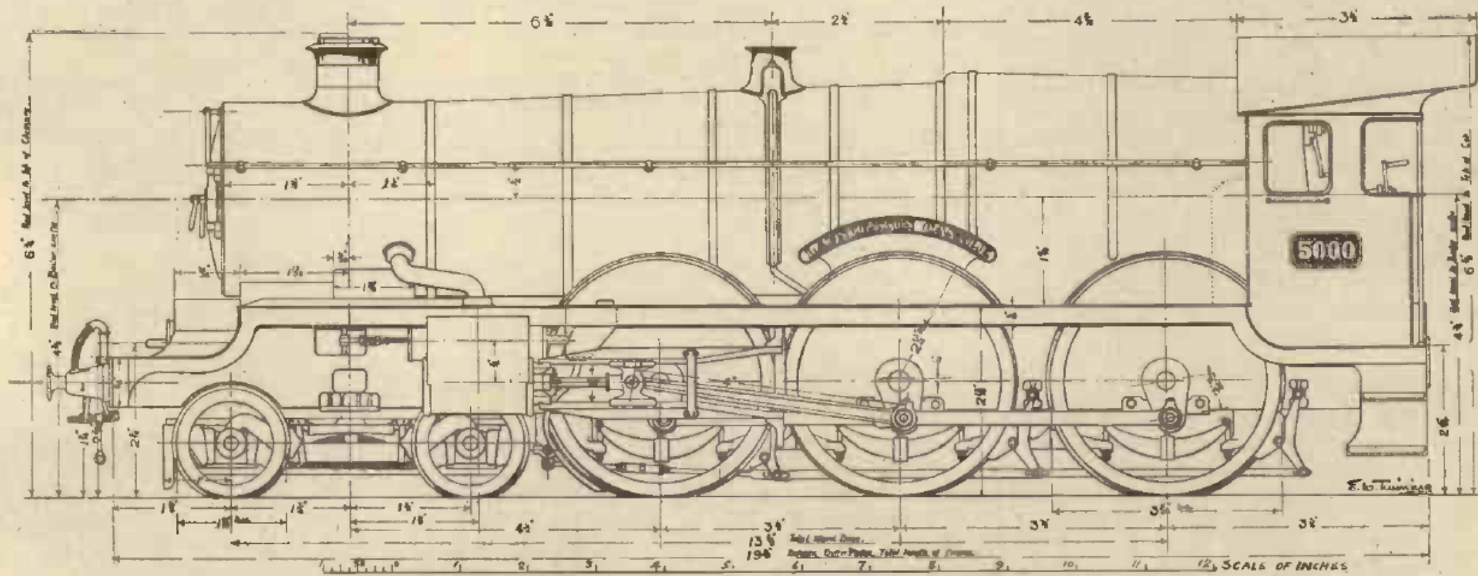
Fig. 1.—An outside elevation of the model, showing the left-hand side.
