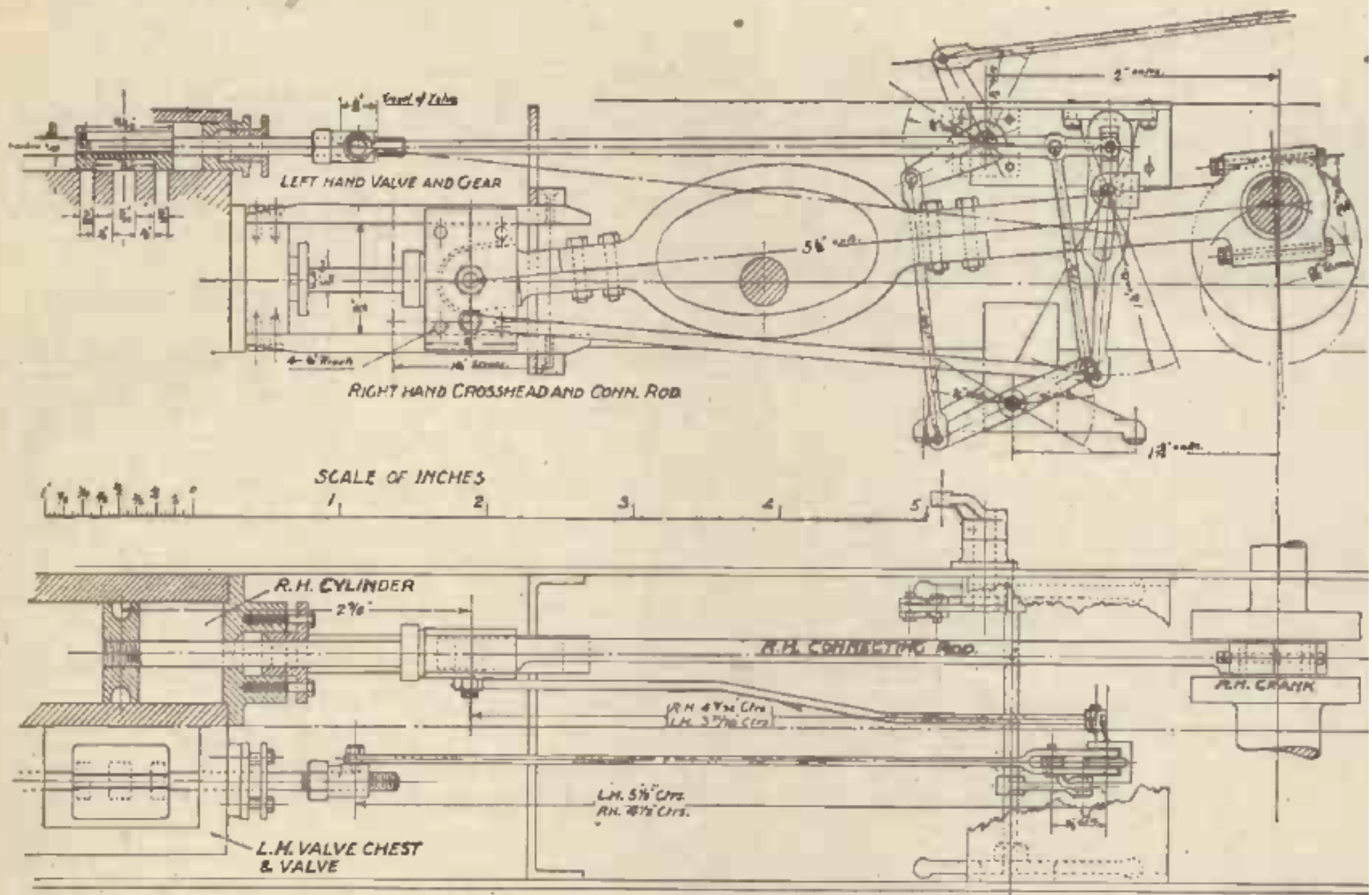
Fig. 4.—An enlarged detailed drawing of the motion and valve gear.
