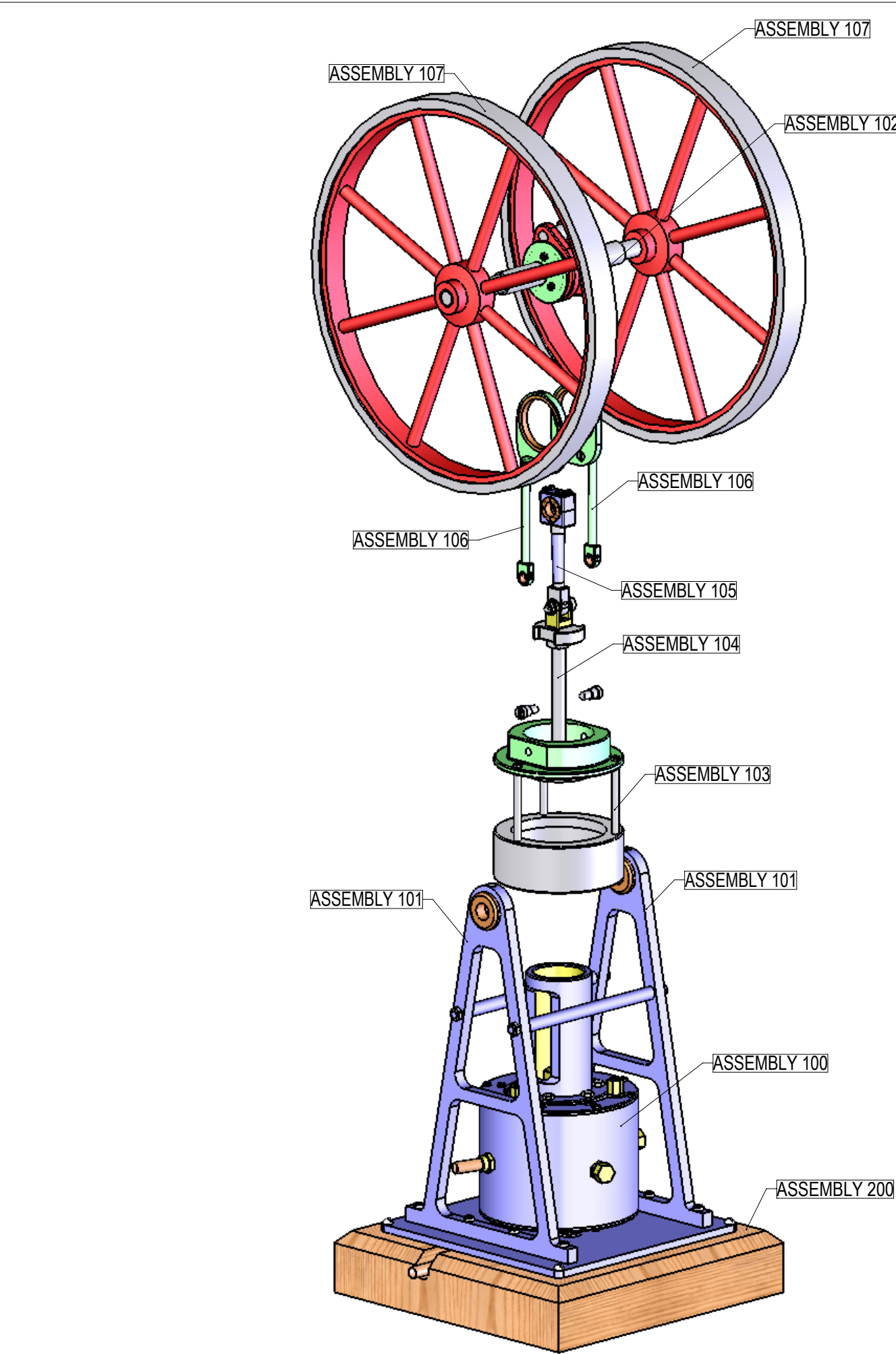
TITLE EXPERIMENTAL VERTICAL SINGLE CYLINDER STEAM ENGINE WITH CIRCULAR VALVE ASSEMBLIES AND PARTS LIST
