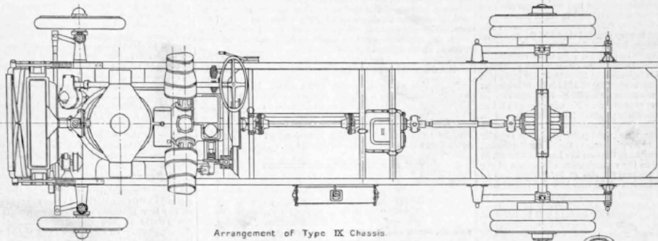
Arrangement of Type IX Chassis
