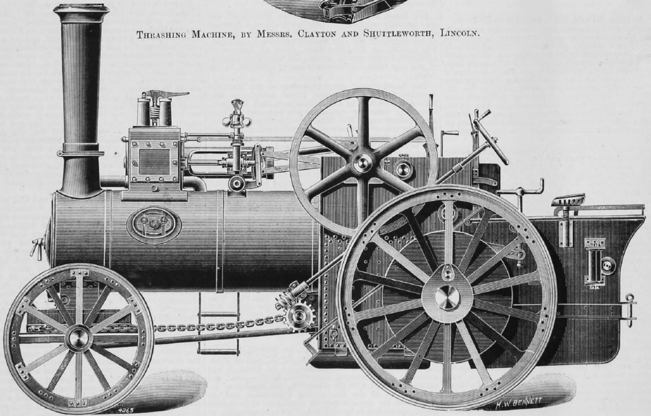
TRACTION ENGINE, BY MESSRS. CLAYTON AND SHUTTLEWORTH, LINCOLN.
