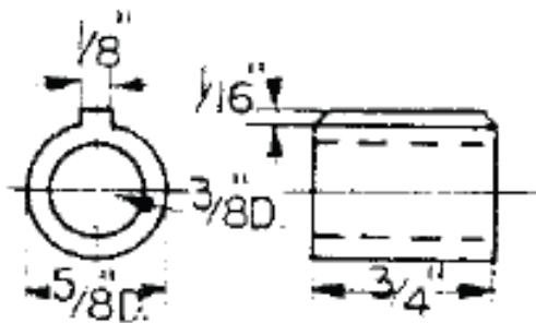
CHANGE WHEEL MOUNTING SLEEVE
