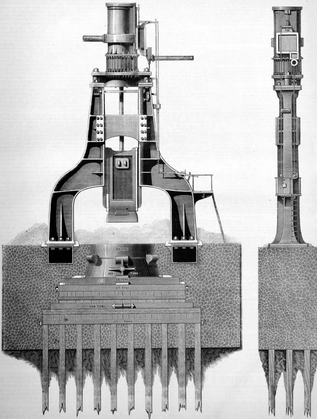
FRONT ELEVATION
