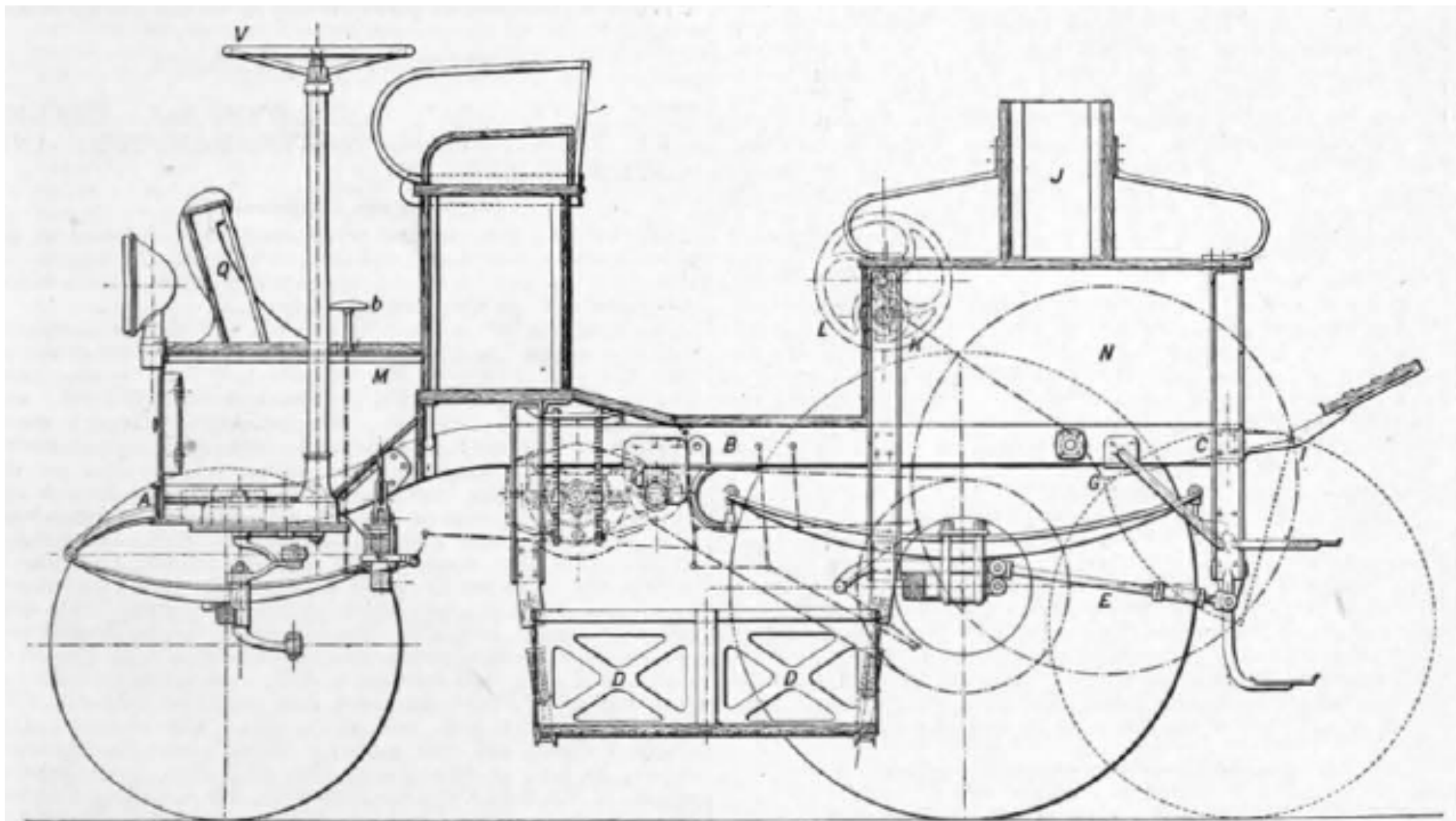
Fig. 2—ELECTRIC FIRE WAGON
