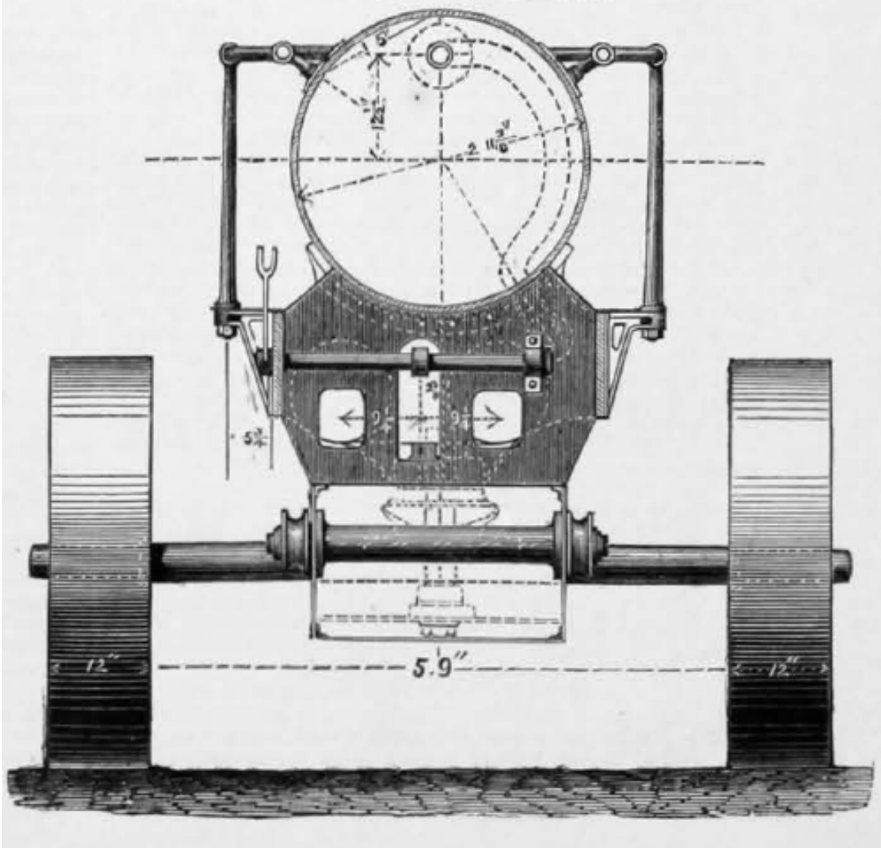
SECTIONAL END ELEVATION
