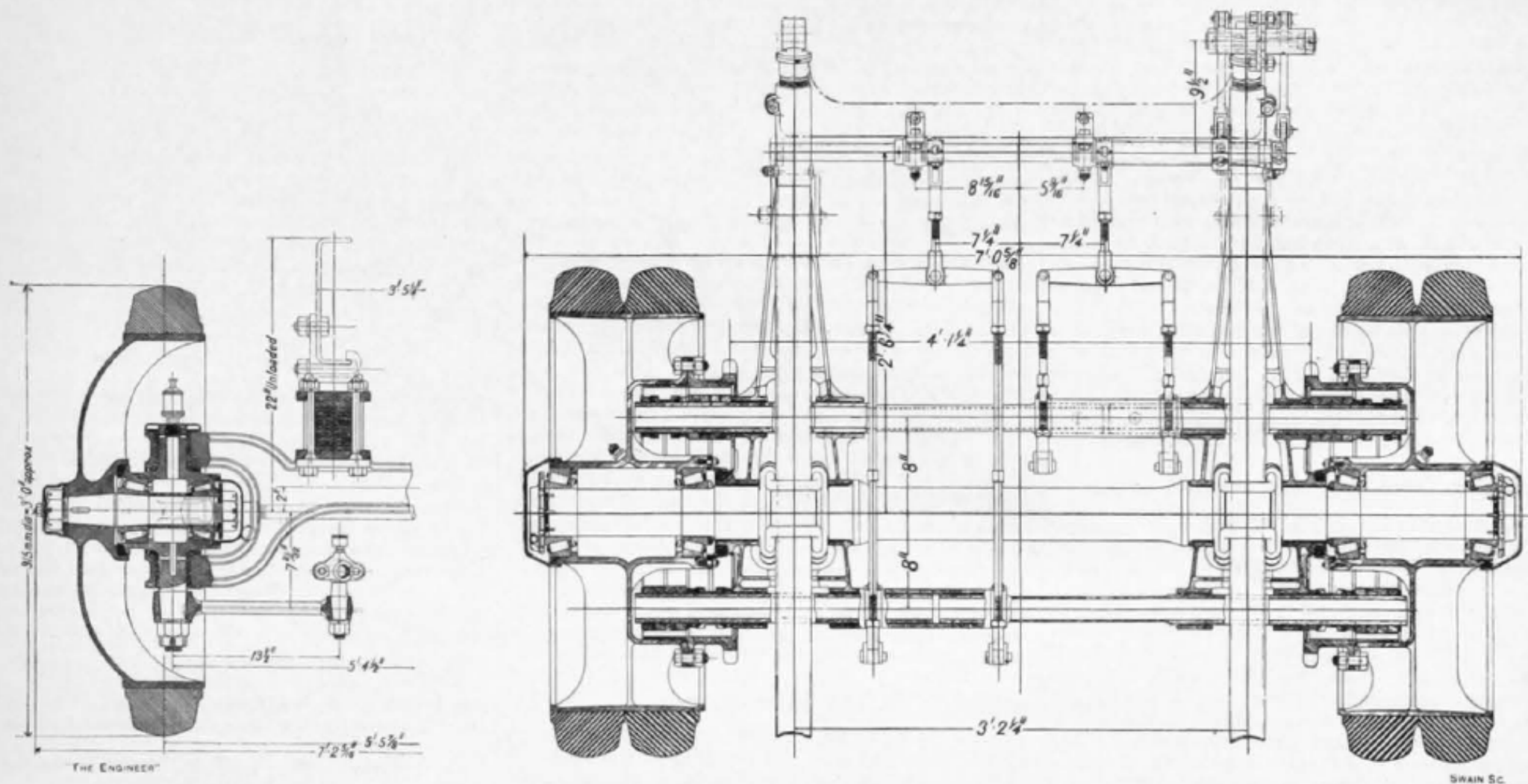
FIG. 1—FRONT WHEEL, BACK AXLE AND BRAKE GEAR
