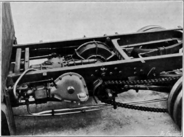
FIG. 4—FEED-PUMP, NEAR SIDE
