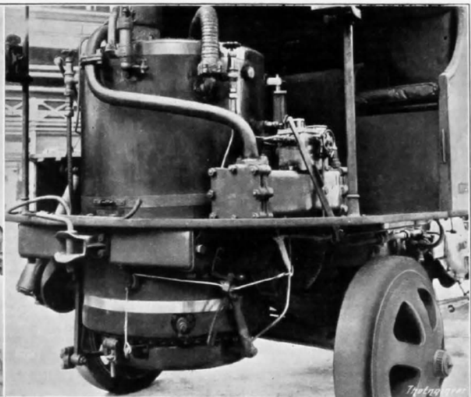
FIG. 8—BOILER, FIREMAN'S SIDE
