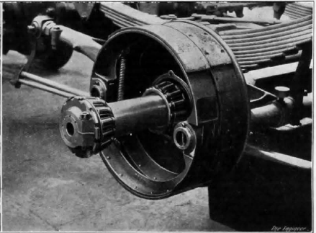
FIG. 6—BRAKE SHOES
