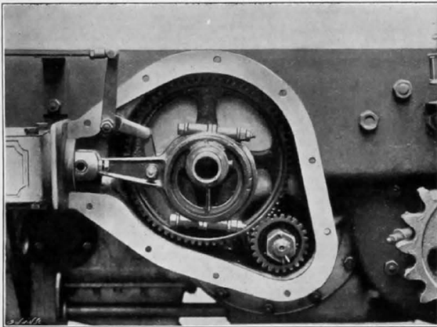
FIG. 5—FEED-PUMP GEARING
