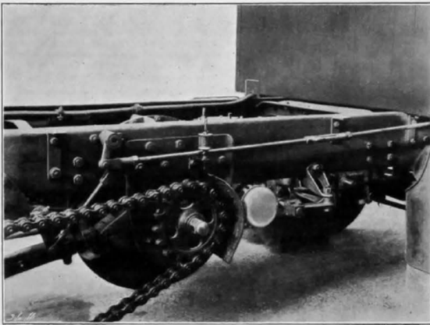
FIG. 3—CHAIN DRIVE ON OFF SIDE
