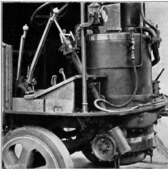
FIG. 7—BOILER, DRIVER'S SIDE
