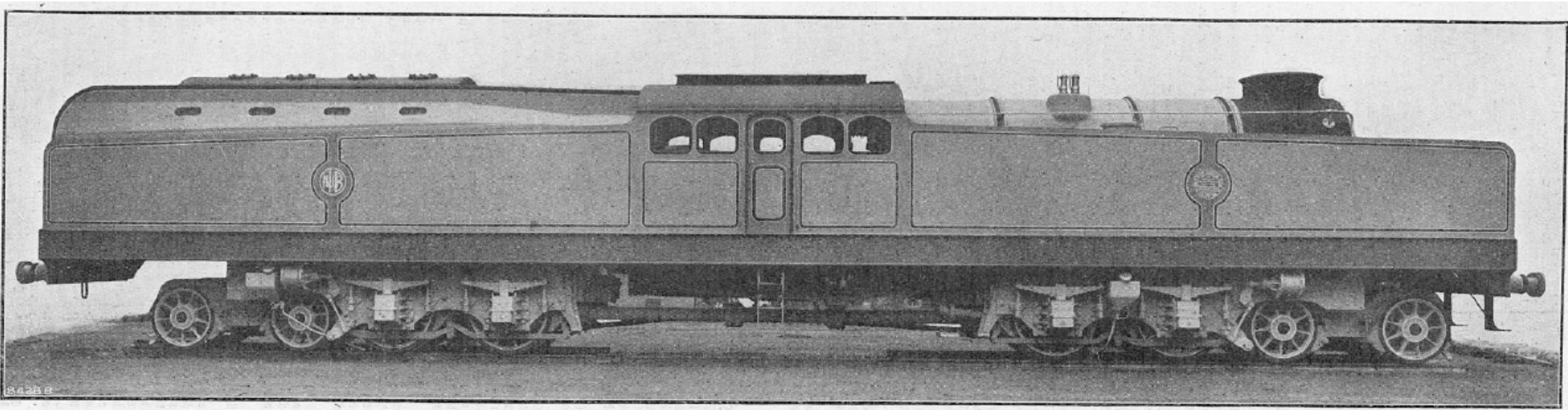
FIG. 188. GENERAL VIEW OF LOCOMOTIVE.
