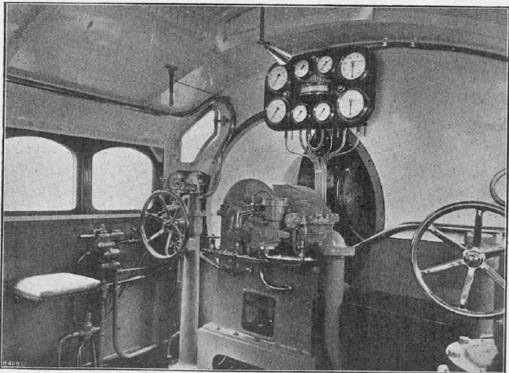
FIG. 190. INTERIOR OF CAB; DRIVER'S END
