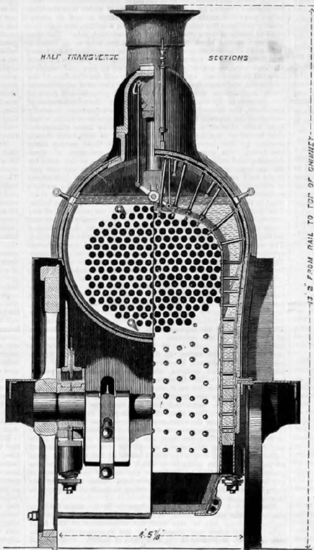
CROSS SECTIONS OF EXPRESS LOCOMOTIVE, L. B. & S. C. RAILWAY.
