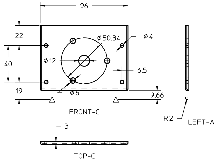
Front Frame
