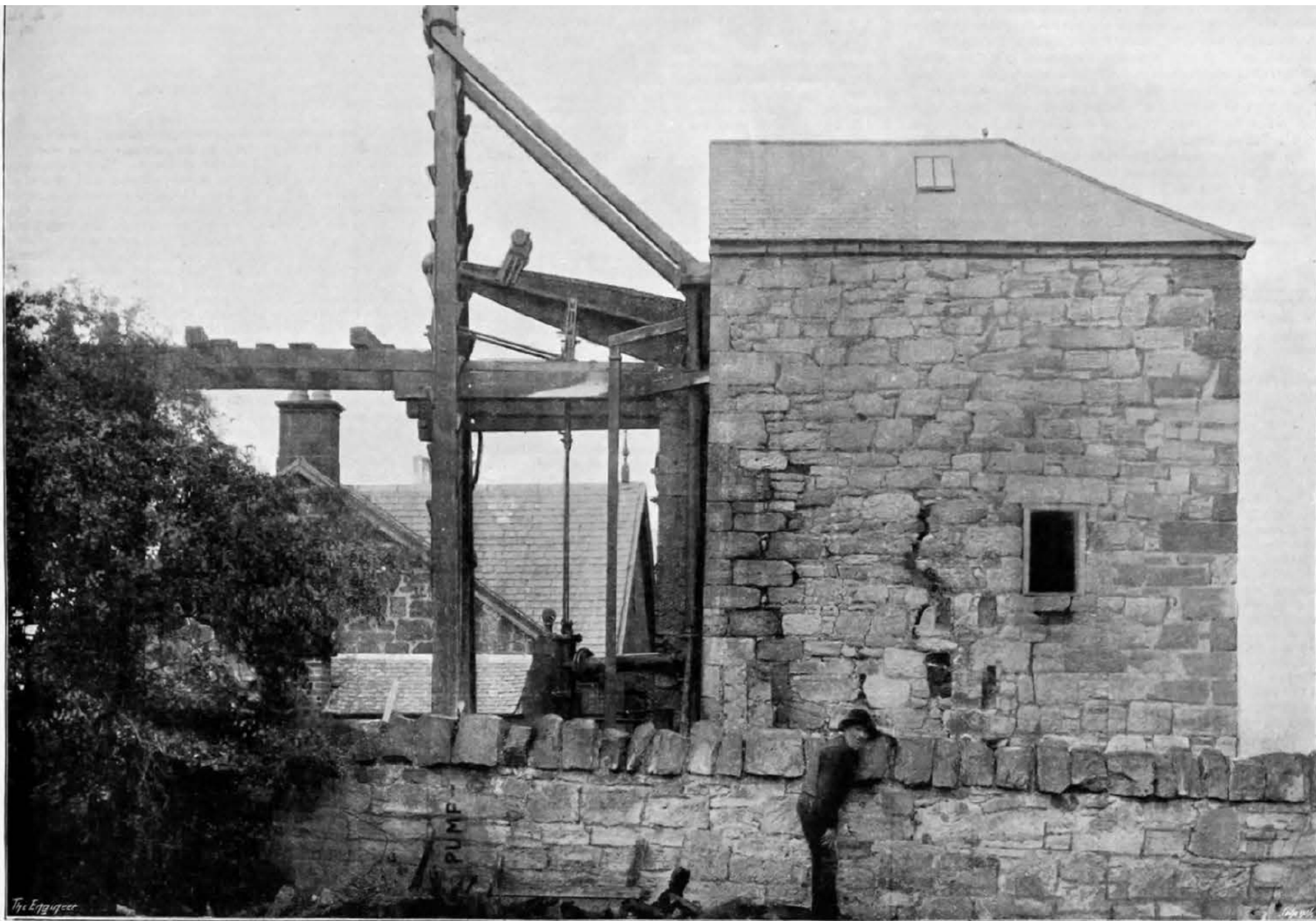
NEWCOMEN ENGINE, CAPRINGTON COLLIERY, KILMARNOCK, 1803
