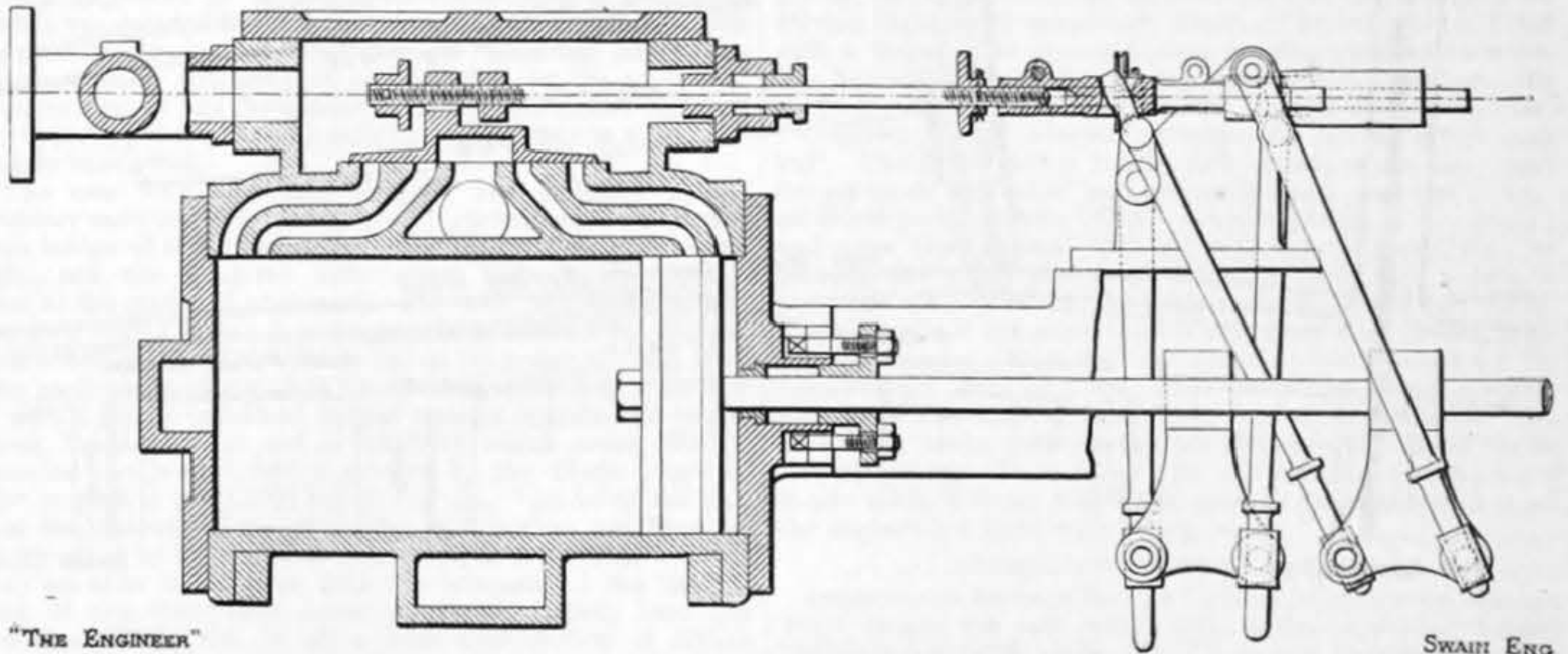
ARRANGEMENT OF VALVES AND VALVE LEVERS, PROSPECT DUPLEX PUMP
