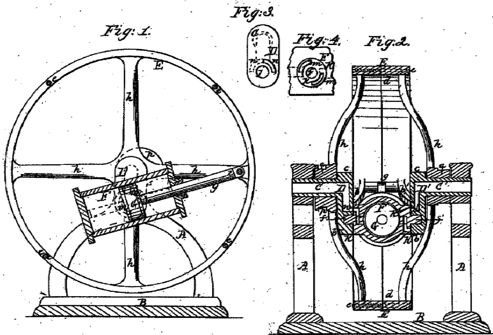
THOMAS ROGERS. REVOLVING CYLINDER STEAM ENGINE No 19,715 PATENTED MAR. 23, 1858
