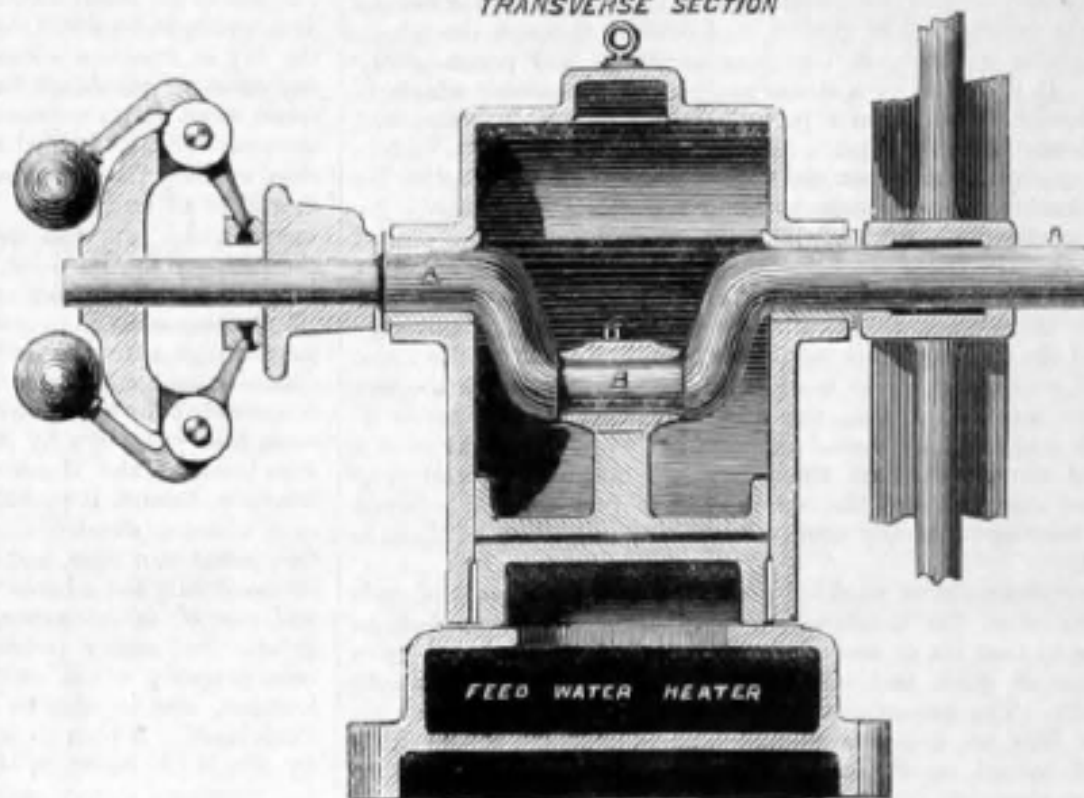
TRANSVERSE SECTION
