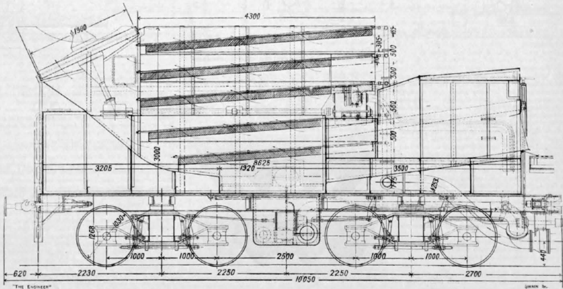
TENDER WITH WATER-COOLING PLANT FOR TURBINE LOCOMOTIVE
