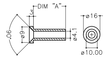
DIM "A" 5.05-5.1 DRILL ROD
