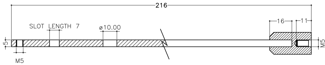
MILD STEEL FABRICATION
