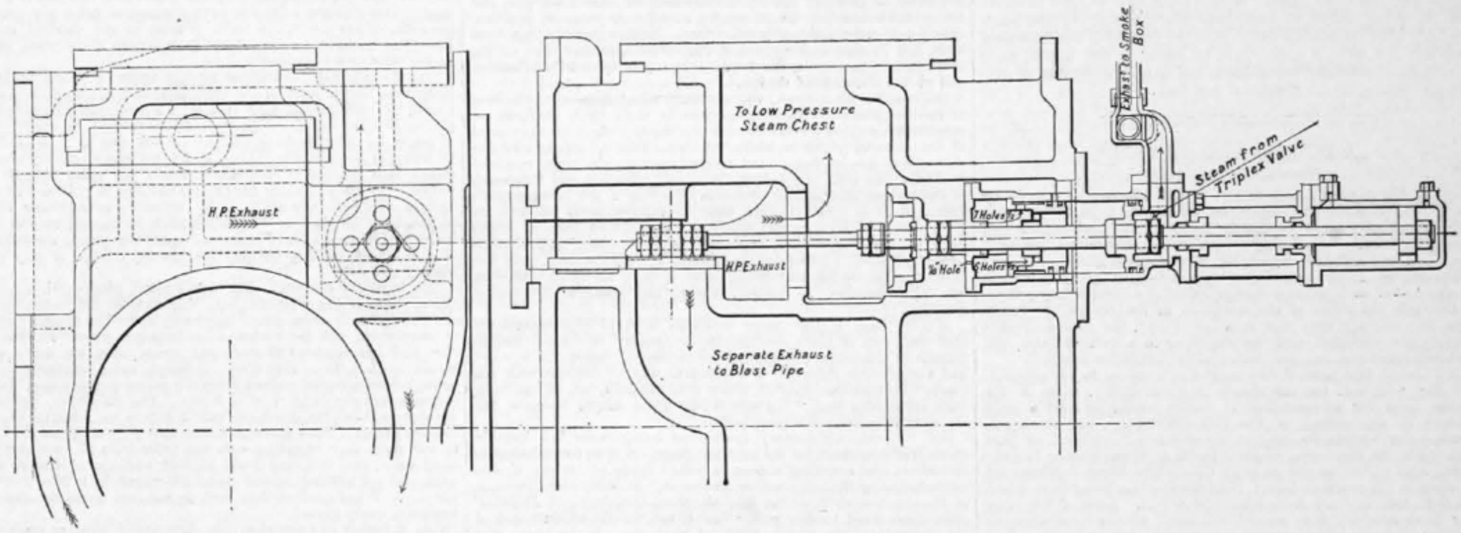
IVATT'S COMPOUND ENGINE CHANGE VALVE
